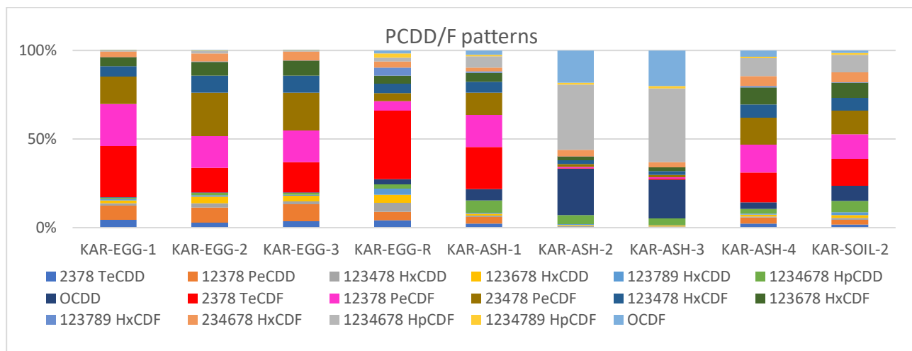
Figure 2: PCDD/F patterns.
